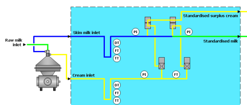
P&I DIAGRAM STANDARDISATION UNIT
